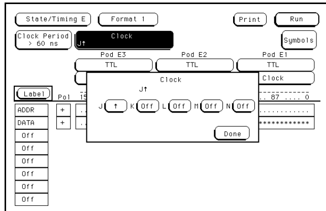
Figure 8-9. Clock Selection
