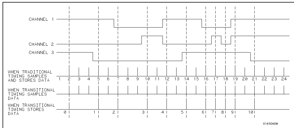
Figure 5-32. Transitional Timing vs. Traditional Timing
