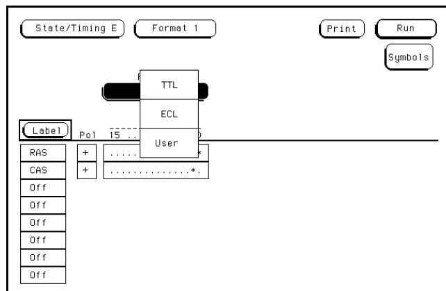
Figure 3 - 3. Pod Threshold
