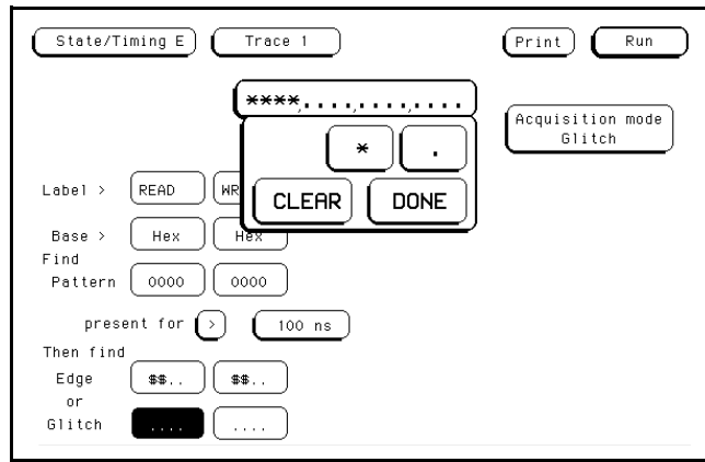
Figure 5-46. Glitches Specified
