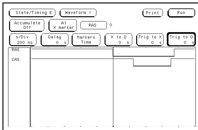
Figure 7-9. Waveform at 200 ns/Div
