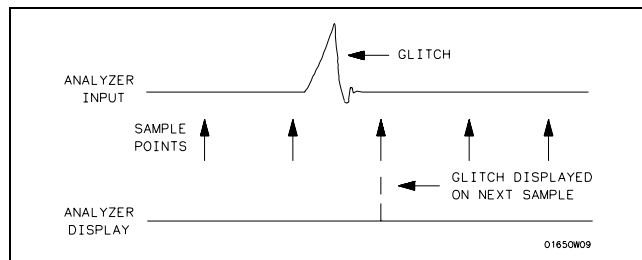
Figure 5-34. Glitch in Timing Waveform
