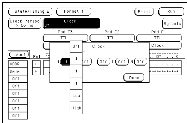
Figure 8-11. Negative-edge Selection
