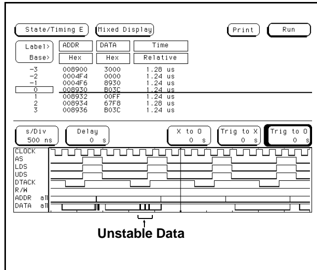
Figure 12-20. Mixed Mode Display with Unstable
