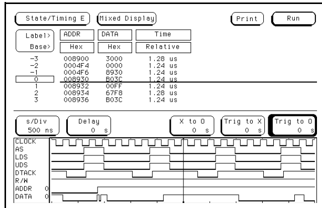
Figure 6-15. Timing/State Mixed Mode Display
