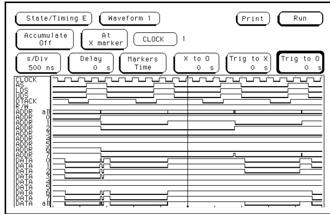
Figure 6-2. Timing Waveforms Menu with 24
