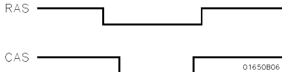
Figure 7-8. RAS and CAS Signals
