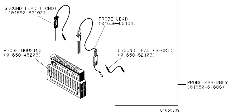
Figure 2-3. Probe Assembly
