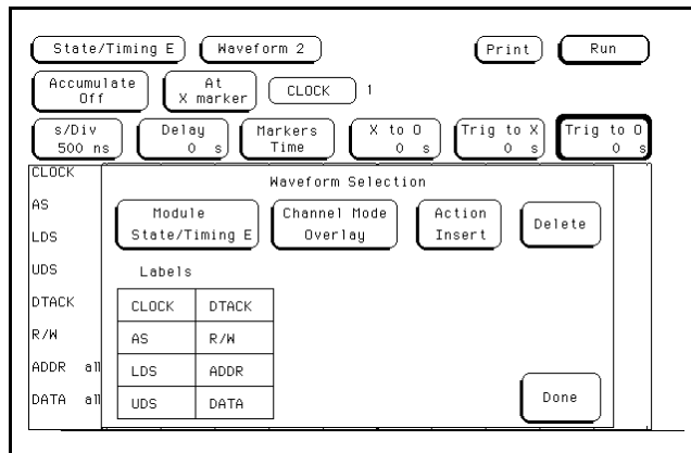
Figure 12-19. Overlapped Waveforms
