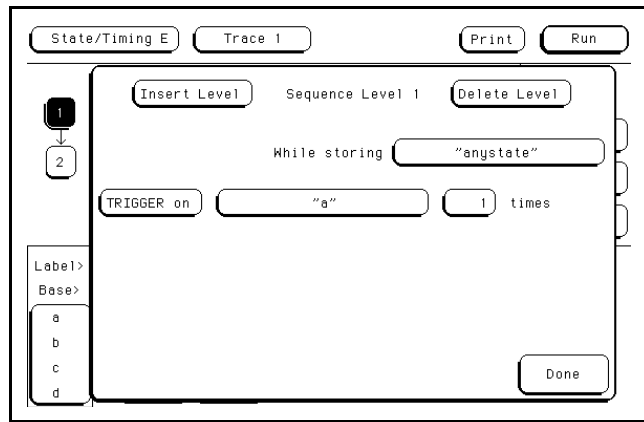
Figure 8-14. Sequence Levels
