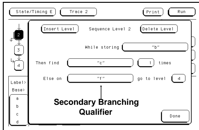
Figure 5-67. Secondary Branching
